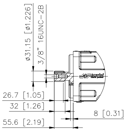
S12 SCANALATO / SPLINED 14T 12/24 DP
